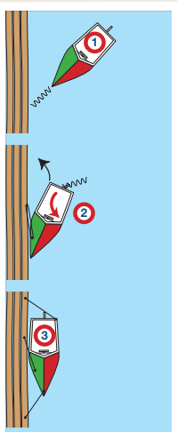
Berthing; single shaft
